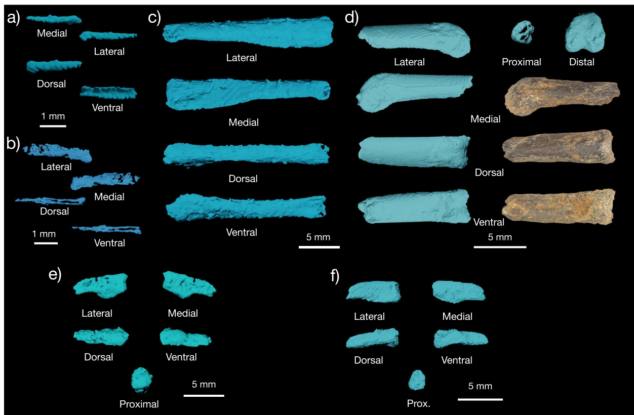
Fig. 6 Pedal elements of YPM VP 59473. Pedal phalanges I-1? (a), I-1? (b), II-1? (c), III-1? (d), III-3? (e), and IV-5? (f) in multiple views. In (d), phalanx is shown in both color illustrations and CT scans
