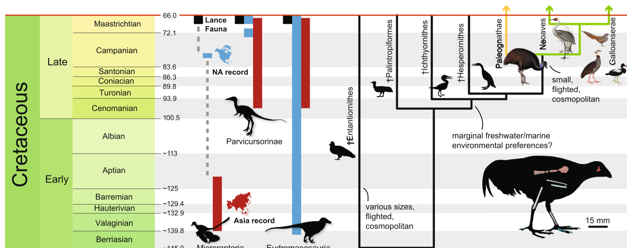
Fig. 7 The ecological and temporal origins of living birds. Left side of the diagram shows the temporal and spatial range extensions and records of key small-bodied non-avian theropod clades found in the Lance Formation assemblage, and cladogram at right shows the major clades of stem and crown birds that survive to or past the K-Pg extinction, with ecologically relevant features that have been considered important to differential avian survival through that event noted along branches. All clades shown on tree are unambiguously represented in the Lance Formation assemblage, except Neoaves and Paleognathae. Divergence times for major lineages are primarily based on [2, 13, 14]. Outlines are public domain from phylopic.org or by the author. Bird illustrations are public domain by John Gould
