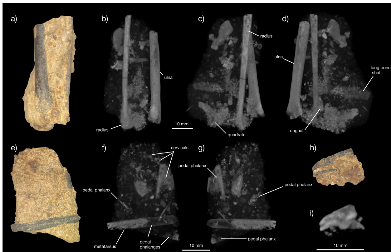
Fig. 1 Preservation of YPM VP 59473. The blocks containing all bones of the holotype (except for the humerus, tibiotarsus, synsacrum fragment, and large distal pedal phalanx) are shown under light microscopy ( a , e , h ) and with multiple x-ray views of the largest ( b , c , d ), second largest ( f , g ), and smallest ( i ) blocks as rendered in VGStudio, showing the relative placement of bones in the matrix blocks
