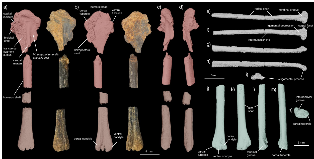
Fig. 3 Forelimb of YPM VP 59473. Humerus in (a) posterior, (b) anterior, (c) lateral, and (d) medial views. In (a) and (b), both CT scans and color images are shown. Radius in (e) anterior, (f) posterior, (g) lateral, (h) medial, and (i) distal views. Ulna in (j) posterior, (k) anterior, (l) lateral, and (m) medial views
